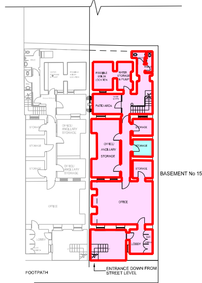
BASEMENT PLAN
